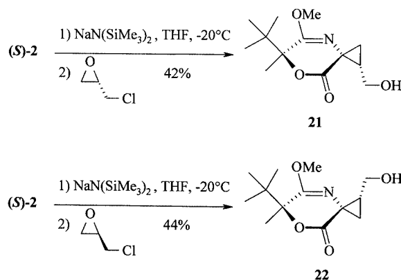
Scheme 6. Direct conversion of ( S )- 2 and ( R )- 2 into 21 and 22 by use of epichlorohydrin
