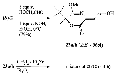
Scheme 7. Cyclopropanation of 23a/b by use of \text{CH}_2\text{I}_2/\text{Et}_2\text{Zn} according to Furukawa
