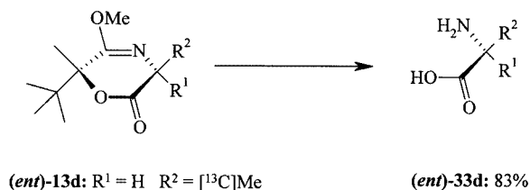
Scheme 10. Hydrolysis of mono- and dialkylated derivatives of 2
