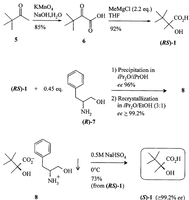
Scheme 2. Preparation of ( S )- 1 by optical resolution of racemic ( RS )- 1
