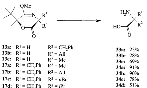
Scheme 11. Hydrolysis of cyclopropyl derivatives to the corresponding free amino acids
