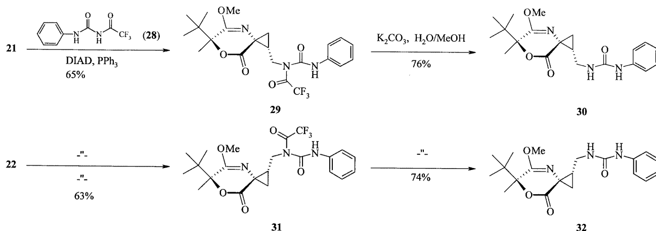
Scheme 9. Preparation of the urea derivatives 30 and 32 by Mitsunobu reaction of 21 and 22 with 1-phenyl-3-(2,2,2-trifluoroacetyl)urea ( 28 ) and subsequent removal of the trifluoroacetyl group by basic hydrolysis
