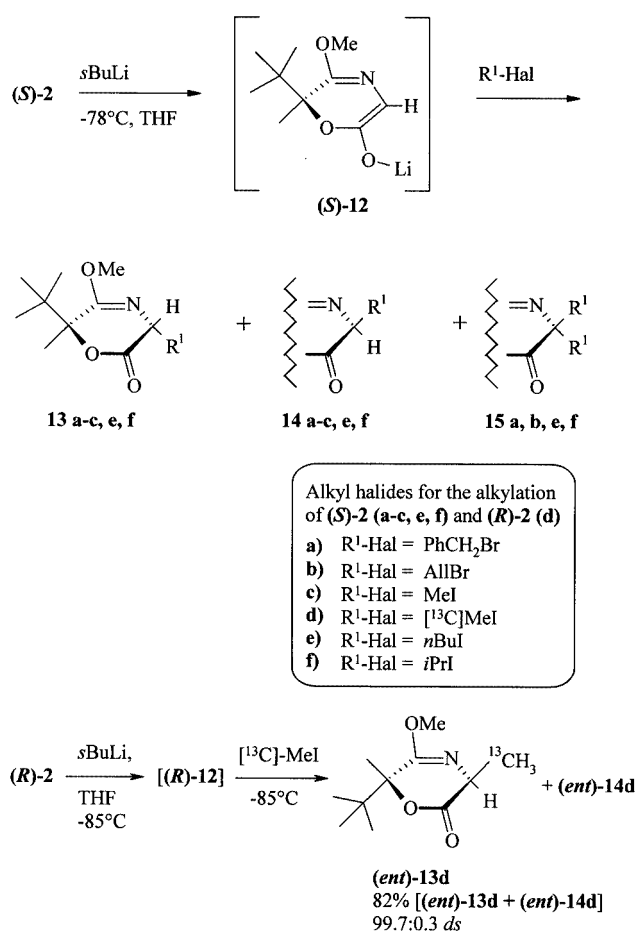
Scheme 4. Alkylation of the oxazinone (S) -2 and (R) -2 via the corresponding enolates
