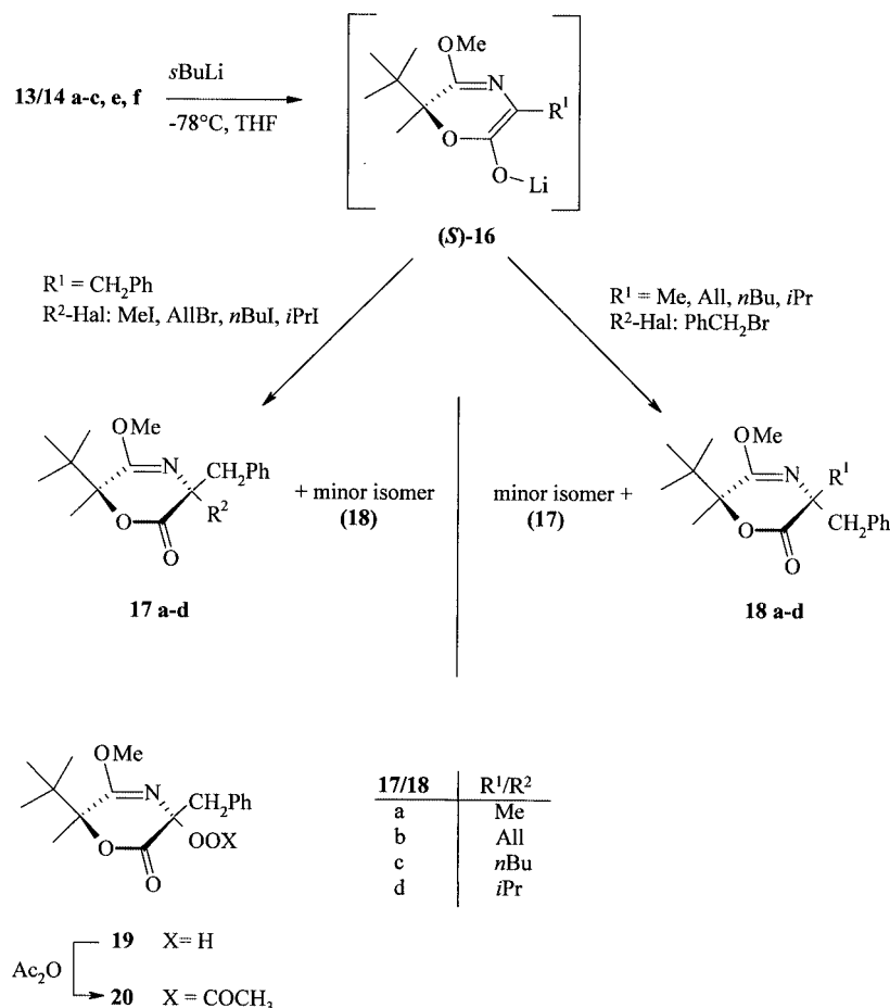
Scheme 5. Second alkylation of the monoalkylation products 13/14 a–c, e, f .
