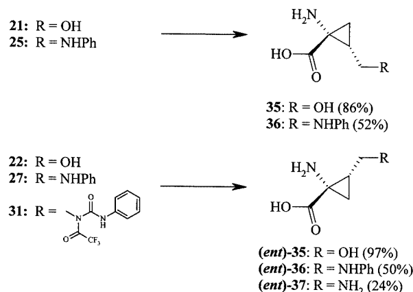
Scheme 11. Hydrolysis of cyclopropyl derivatives to the corresponding free amino acids
