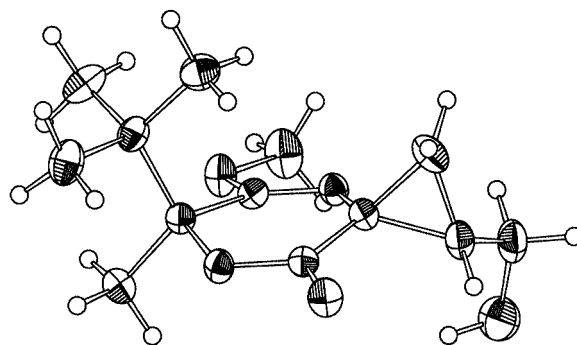
Figure 1. X-ray diffraction analysis of 21
