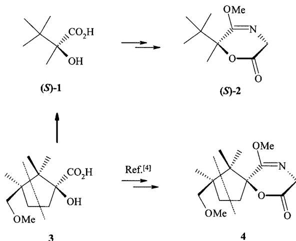
Scheme 1. Delineation of the chiral glycine equivalent ( S )- 2 from 4
