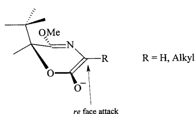
Scheme 12. Hypothetical model for the asymmetric induction in the alkylation reactions of the enolates ( S )- 12 and ( S )- 16
