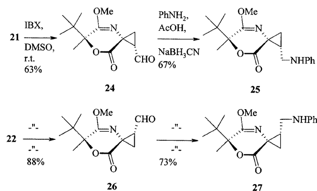
Scheme 8. Oxidation and subsequent reductive amination of 21 , and 22 to the corresponding aniline derivatives. IBX = ortho -iodoxybenzoic acid
