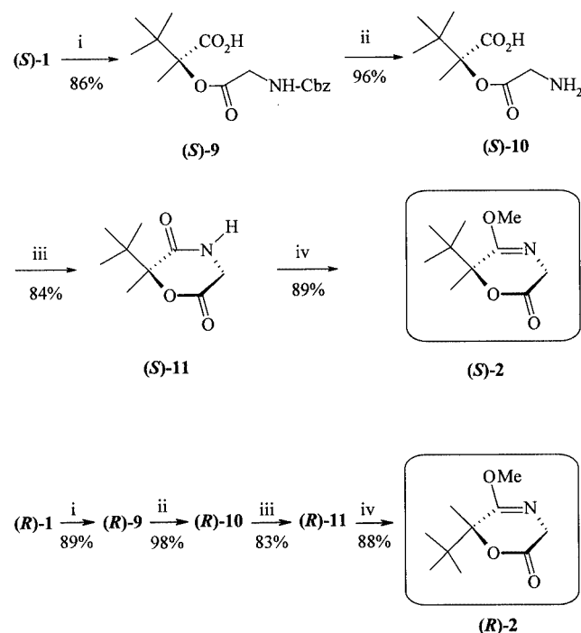
Scheme 3. Synthesis of the chiral glycine equivalents ( S )-2 and ( R )-2: i) Cbz-glycine, CDI, THF; ii) H 2 , Pd/C, EtOH; iii) 2-chloro-1-methylpyridinium iodide, i Pr 2 EtN, CH 2 Cl 2 ; iv) Me 3 O + BF 4 − , CH 2 Cl 2
